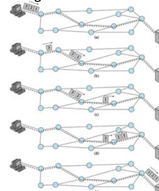
Figure 10.10 Packet Switching: Virtual-Circuit Approach
