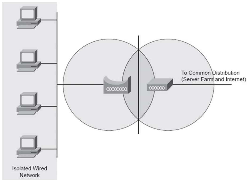
Workgroup Bridge Topology
