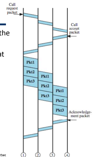
(b) Virtual circuit packet switching
