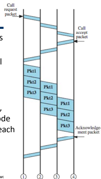
(b) Virtual circuit packet switching
