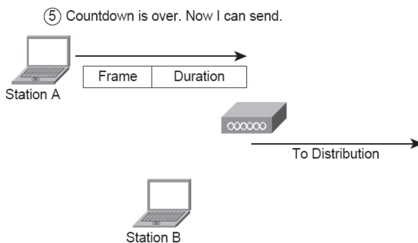
Sending a Frame: Part 2
